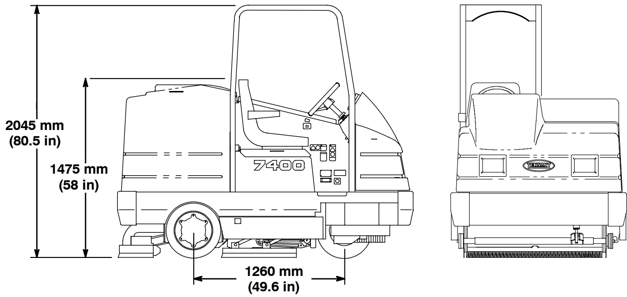
MACHINE DIMENSIONS
